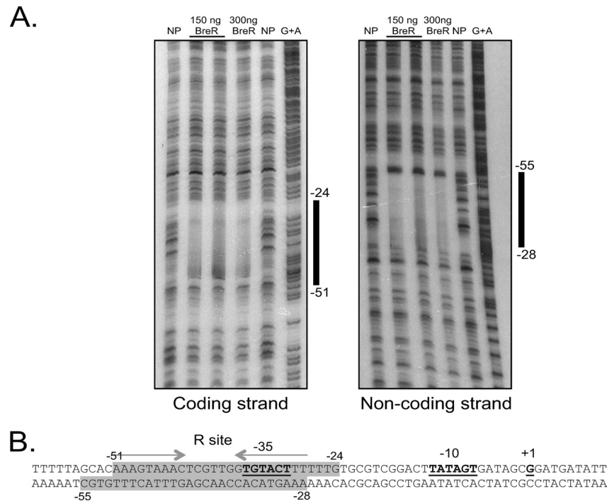
FIG 2 DNase I protection of the breR promoter by BreR. (A) The coding and noncoding strands of the ^{32}\text{P} -end-labeled fragment from positions -158 to +81 were incubated with a 1:200 dilution of DNase I and no protein (NP; lanes 1 and 5), \sim 150 ng BreR and a 1:200 DNase I dilution (lane 2) or a 1:400 DNase I dilution (lane 3), \sim 300 ng BreR and a 1:200 dilution of DNase I (lane 4), and a G+A sequencing reaction (lane 6). The region of protection by BreR is indicated with a black bar. (B) Double-stranded DNA sequence showing the BreR-protected region at the breR promoter. The protected region for both strands is shaded in gray, and the endpoints of the protection above and below the shaded regions are labeled ( -55 to -24 ). A region with partial dyad symmetry, involved in DNA binding, is indicated by gray arrows. The transcriptional start site ( +1 ) (17) and putative -35 and -10 regions are highlighted in boldface and are underlined.
