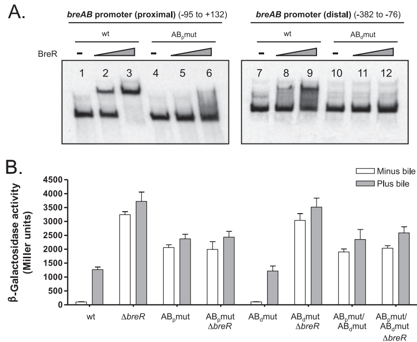
FIG 7 Mutational analysis of the AB_p and AB_d binding sites at the breAB promoter. (A) Binding of BreR to the wild-type and mutated ( AB_p mut and AB_d mut) AB_p and AB_d fragments. EMSA was performed using DIG-dUTP-labeled DNA (10 ng) incubated with 0 (lanes 1, 4, 7, and 10), 50 (lanes 2, 5, 8, and 11), or 250 ng (lanes 3, 6, 9, and 12) of BreR-His 6 prior to electrophoresis. (B) Influence of base pair mutations in P_{breAB} - lacZ expression in various strain backgrounds. \beta -Galactosidase activity was measured as described for Fig. 6.
