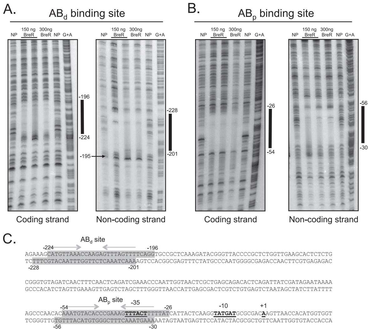
FIG 4 DNase I footprinting analyses for BreR at the breAB promoter. The coding and noncoding strands of two radioactively 33 P-end-labeled fragments of 230 bp (–327 to –97) (A) and 246 bp (–167 to +78) (B) were incubated with a 1:200 dilution of DNase I and no protein (NP; lanes 1 and 5), ~150 ng BreR and a 1:200 DNase I dilution (lane 2) or a 1:400 DNase I dilution (lane 3), ~300 ng BreR and a 1:200 dilution of DNase I (lane 4), and a G+A sequencing reaction (lane 6). The region of protection by BreR and a region of hypersensitivity induced by BreR are indicated by thick black lines and a black arrow, respectively. (C) Double-stranded DNA sequence of the breAB promoter. BreR-protected regions are shaded in gray for both strands. Regions of partial dyad symmetry, involved in DNA binding, are shown for the AB d and AB p binding sites with gray arrows. The transcriptional start site (+1) (17), ATG start codon, and putative –35 and –10 regions are highlighted in boldface and are underlined.
